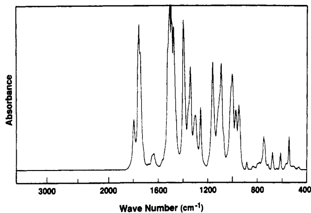
Figure 2. Infrared spectrum of a 10FEDA/4FMPD film.
