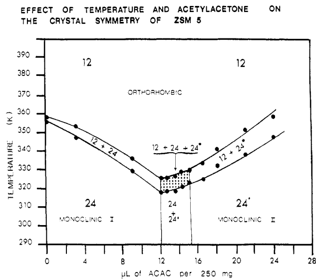
Figure 12. Phase diagram showing the relationship between the three observed phases (monoclinic I, monoclinic II and orthorhombic) with variation of temperature and the concentration of acetylacetone. All three phases coexist in the central region of the diagram.
