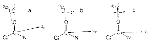
Figure 8. Orientation of the principal axes of the observed and calculated ^{13}\text{C} chemical shift tensors of glycol residue carbonyl carbon in (a) glycylglycine-HCl·H 2 O, 38 (b) model A (1-type hydrogen bond), and (c) model B (2-type hydrogen bond), respectively. The direction of \sigma_{33} (not shown here) is perpendicular to the directions of \sigma_{11} and \sigma_{22} .
