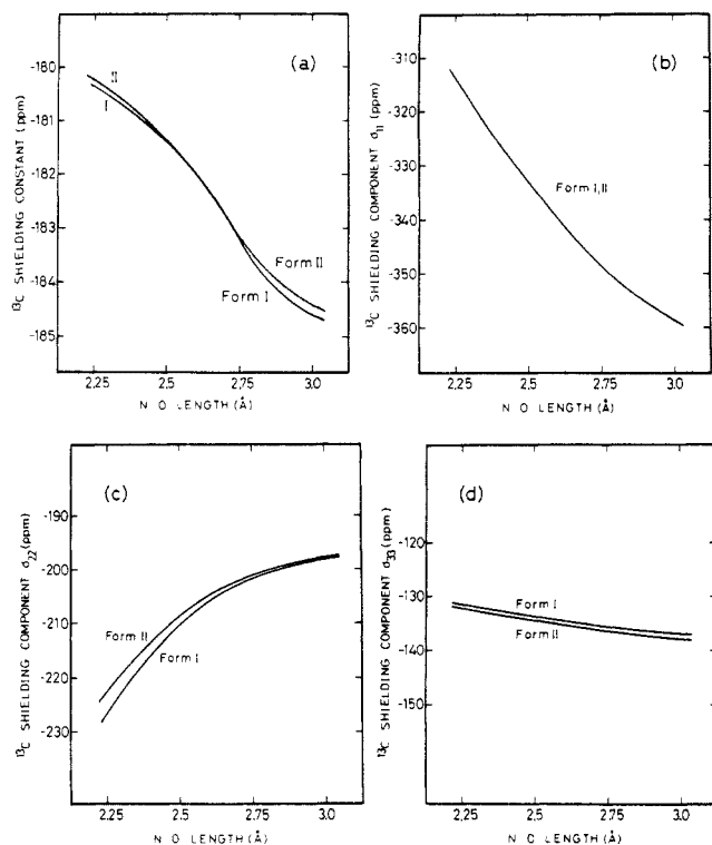
Figure 6. Variation of the calculated ^{13}\text{C} shielding constant and its tensor components with the N...O hydrogen bond length ( R_{\text{N}\cdots\text{O}} ) for the 2-type hydrogen bond: (a) isotropic shielding constant and (b) \sigma_{11} , (c) \sigma_{22} , and (d) \sigma_{33} .
