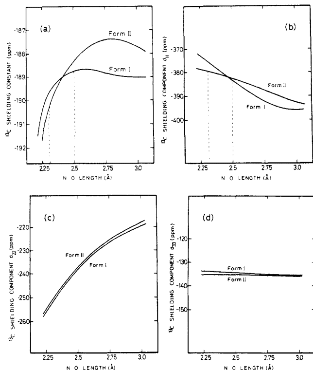
Figure 5. Variation of the calculated ^{13}\text{C} shielding constant and its tensor components with the N...O hydrogen bond length ( R_{\text{N}\cdots\text{O}} ) for the 1-type hydrogen bond: (a) isotropic shielding constant and (b) \sigma_{11} , (c) \sigma_{22} , and (d) \sigma_{33} .
