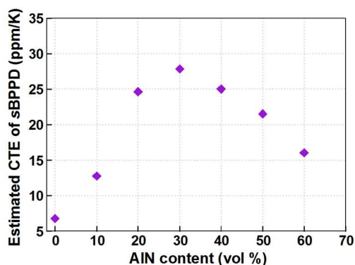
Fig.10 Estimated CTE of sBPPD matrix in the presence of AIN particles
