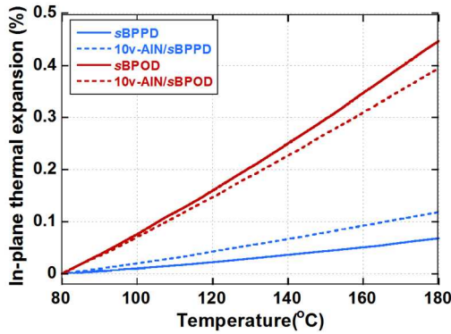
Fig.7 TMA curves of pristine PIs and 10v-AIN/PIs.
