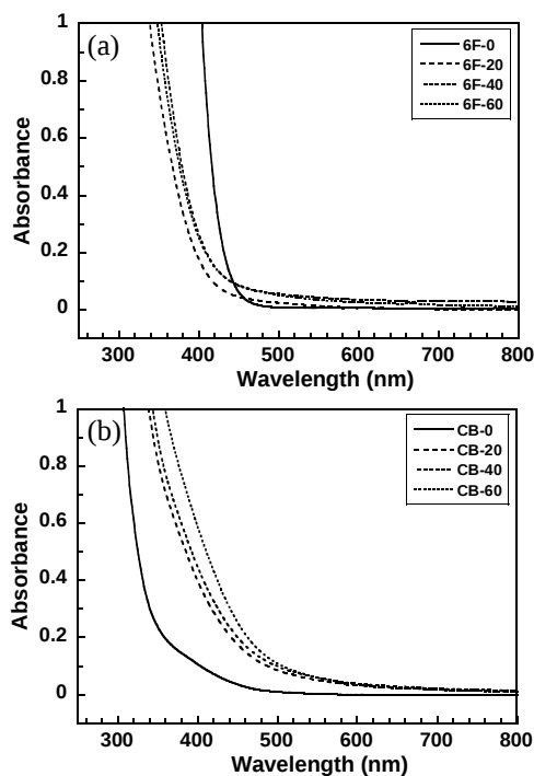
Fig. 7 UV-vis spectra of DEN/PI hybrid films: (a) DEN/6FDA-ODA and (b) DEN/CBDA-ODA.
