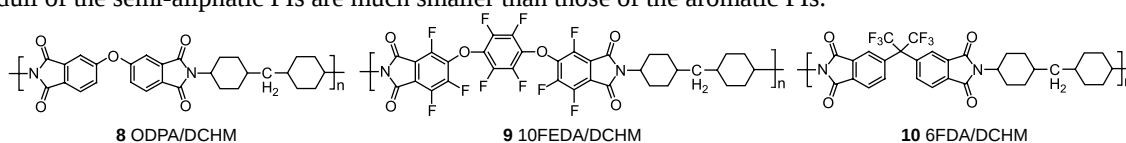
Fig. 6 Molecular structures of semi-aliphatic polyimides used in this study.
