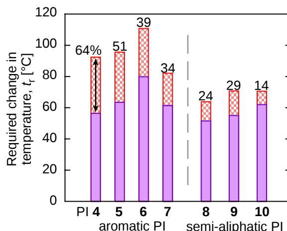
Fig. 7 Polarization dependence in the calculated values of required temperature changes t_r for 0.3% decreases in refractive indices. Filled (blue) bars and hashed (red) bars represent the values of t_r for TE- and TM-polarized light, respectively. Numbers placed above the bars represent the excess of t_r^{TM} compared to t_r^{TE} .
