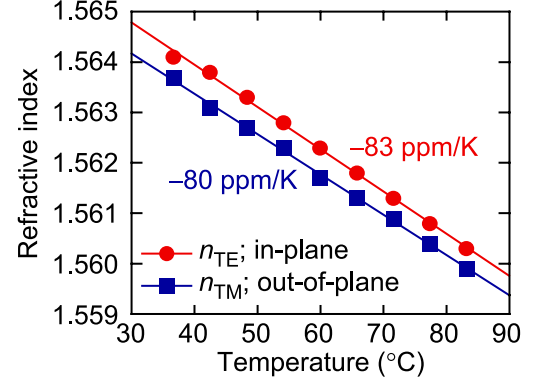
Fig. 5 Temperature dependence of refractive index for the peeled film of PI 7.
