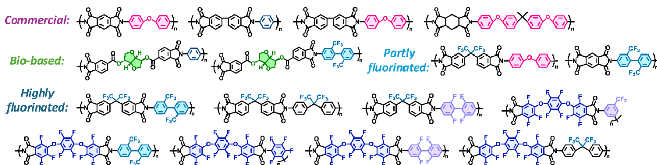
Figure 1. Chemical Structures of 16 types of polyimides.
