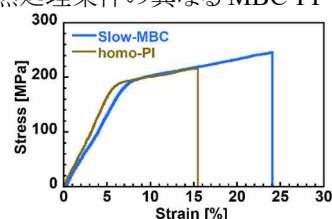
Fig. 2 Mechanical property of homo-PI and Slow-MBC.
