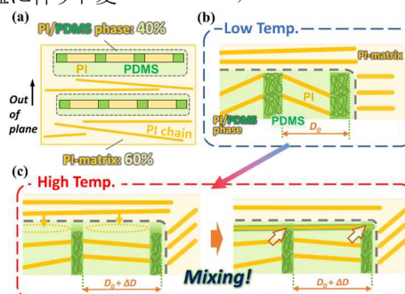
Fig. 4 Schematic models of (a) phase separation and (b)(c) temperature-induced phase mixing mechanism model in MBC-PI.
