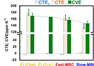
Fig. 3 Thermal deformations of film and crystalline homo-PI, Fast-MBC, and Slow-MBC.
