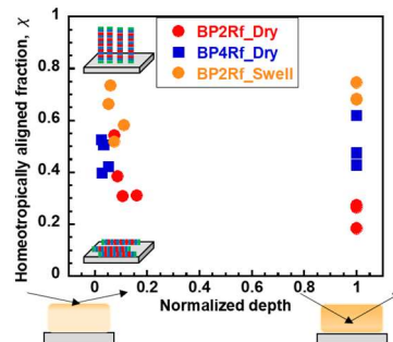
Fig. 3 Depth dependence of volume fraction of the homeotropically aligned domain of BP2Rf, BP4Rf and BP2Rf-PAEs using swelled PDMS films.
