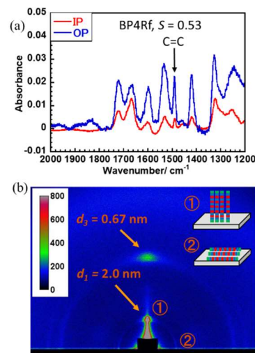
Fig. 2 (a) pMAIRS spectra and (b) 2D GI-WAXD image of a BP4Rf-PAE thin film.
