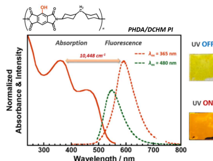
Fig. 1 Photograph and excitation/emission spectra of PHDA/DCHM PI homopolymer
