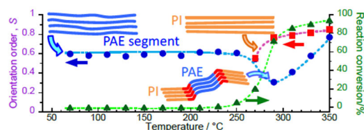
Fig. 2 Temperature evolution of S value of precursor and PI segments. Schematic drawings for the mechanism of orientation enhancement are inset.
