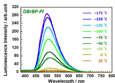
Fig.3. Photoluminescence emission spectra of DBrBP-PI films at low temperatures excited at 367 nm.
