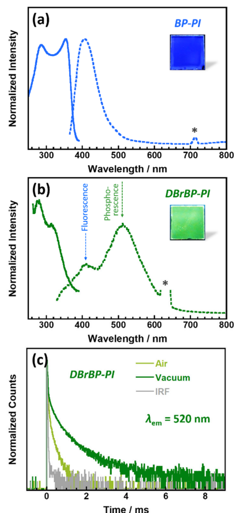
Fig.2. Excitation and emission spectra of (a) BP-PI and (b) DBrBP-PI, and (c) emission delay curves of DBrBP-PI. The msec-order lifetime of DBrBP-PI indicates room temp. phosphorescence (RTP).
