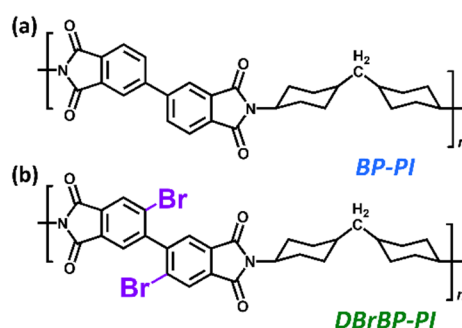
Fig.1. (a) BP-PI & (b) DBrBP-PI.
