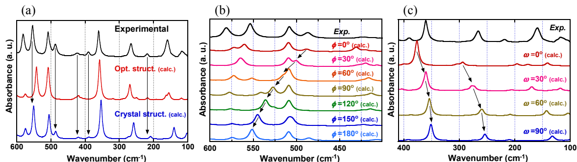
Figure 2. Far-IR spectra of imide model compound (a) top ; experimental, middle ; calculated with optimized structure, bottom ; calculated by assuming crystal structure, and calculated Far-IR spectra of sBPDA-An with variable dihedral angles (b) \phi and (c) \omega .
