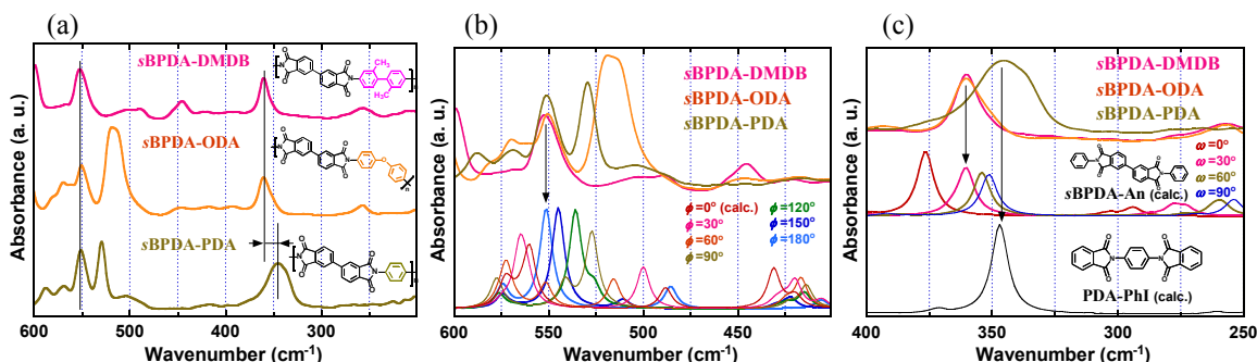
Figure 4. Far-IR spectra of PIs (a) top ; sBPDA-DMDB middle ; sBPDA-ODA, bottom ; sBPDA-PDA (b) top ; experimental spectra of PIs, bottom ; calculated with varying dihedral angle \phi (c) top ; experimental spectra of PIs, middle ; calculated with varying dihedral angle \omega , bottom ; calculated spectra of PDA-PhI.
