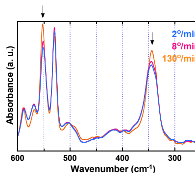
Figure 6. Experimental Far-IR spectra of sBPDA-PDA PI films cured at different heating rates during imidization.
