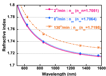
Figure 5. Refractive indices of sBPDA-PDA PI films cured at different heating rates during imidization.
