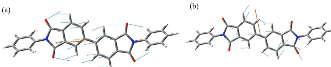
Figure 3. Vibrational modes of imide model compound calculated at (a) 360\text{ cm}^{-1} and (b) 550\text{ cm}^{-1} .
