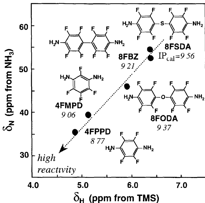
Figure 14.4. 15 N- and 1 H-NMR chemical shifts and calculated ionization potentials (eV) of perfluorinated diamines
