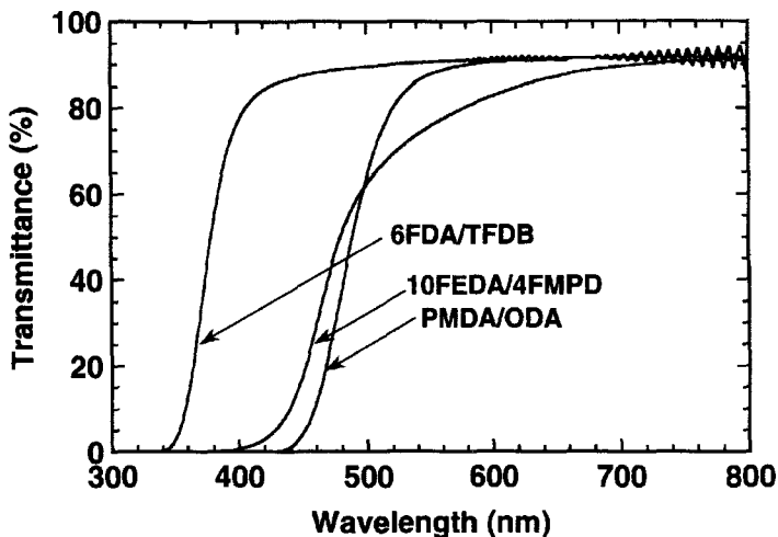
Figure 14.13. UV-visible transmission spectra of partially fluorinated (6FDA/TFDB), perfluorinated (10FEDA/4FMPD), and unfluorinated polyimide (PMDA/ODA) films
