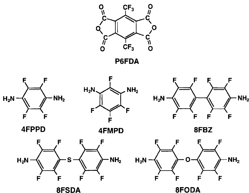
Figure 14.3. Structures of a dianhydride and diamines that can be used for perfluorinated polyimide synthesis (reproduced by permission of the American Chemical Society, from Ando et al. 28 )
