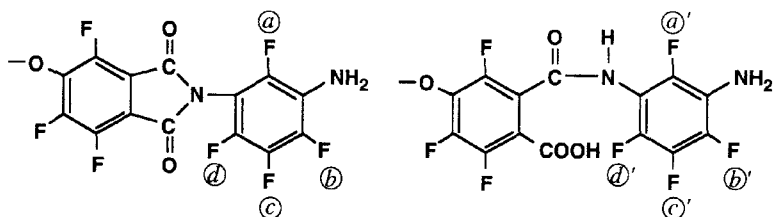
Figure 14.10. Amine-terminal structure of 10FEDA/4FMPD polyimide
