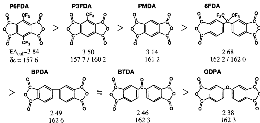
Figure 14.7. Aromatic dianhydrides arranged in order of calculated electron affinity ( E_{A,cal} ) and ^{13}\text{C} -NMR chemical shift of carbonyl carbon ( \delta_C ). Larger E_{A,cal} and smaller \delta_C correspond to the strong electron-accepting property of a dianhydride
