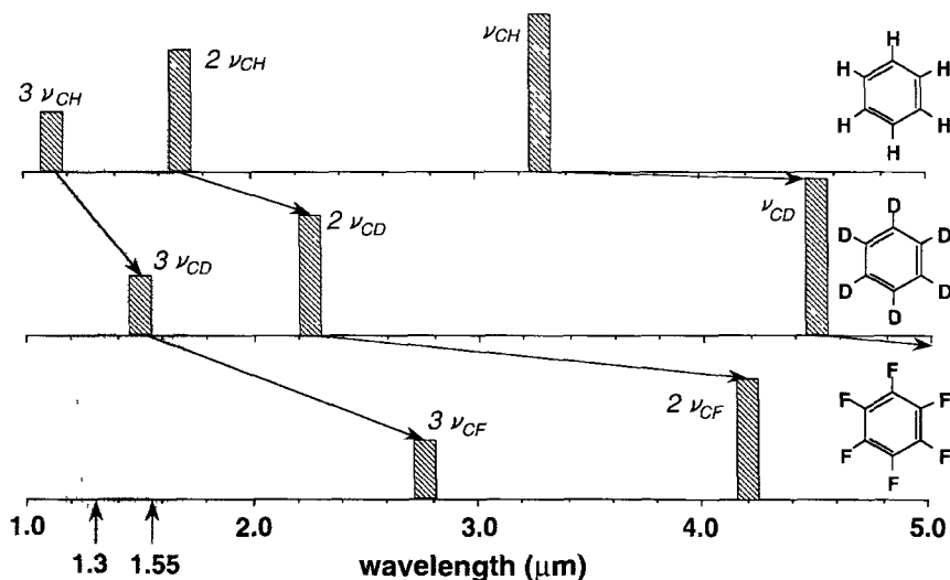
Figure 14.2. Schematic representation of fundamental stretching bands and their harmonic absorption wavelengths for C–H, C–D, and C–F bonds observed for benzene, hexadeuterobenzene, and hexafluorobenzene, respectively (reproduced by permission of the American Chemical Society, from Ando et al. 28 )
