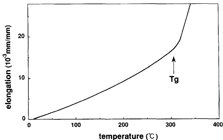
Figure 14.8. Thermal mechanical analysis (TMA) curve of 10FEDA/4FMPD film cured at 350^\circ\text{C} (reproduced by permission of the American Chemical Society, from Ando et al. 28 )
