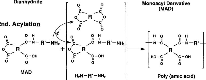
Figure 14.5. Two-step acylation reactions that generate poly(amic acid) from diamine and tetracarboxylic acid dianhydride (reproduced by permission of the American Chemical Society, from Ando et al. 28 )
