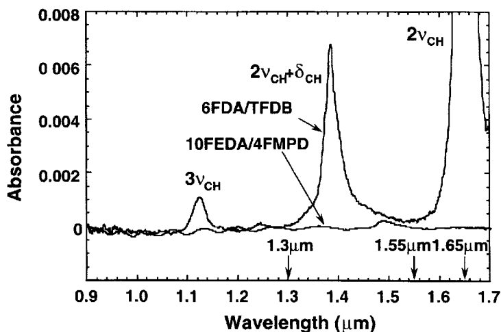
Figure 14.12. Visible-near-IR absorption spectra of 10FEDA/4FMPD and 6FDA/TFDB polyimide films
