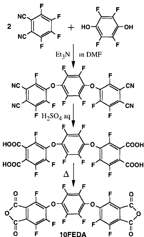
Scheme 1. Synthesis of 10FEDA dianhydride
