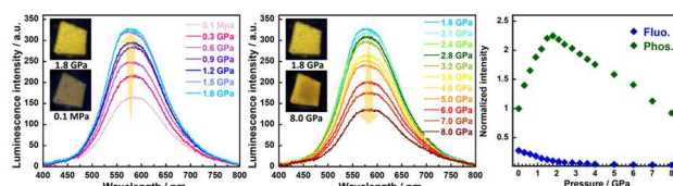
Fig. 2 Pressure-dependent emission spectra of TA-MC/PMMA film and emission intensity.
