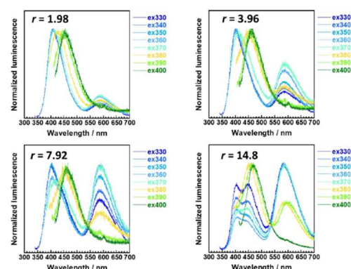
Fig. 4 Normalized fluorescence spectra of ODDC-TsAPA ( r = 1.98, 3.96, 7.92, 14.8 ) observed with different excitation wavelengths ( \lambda_{\text{ex}} = 330, 340, 350, 360, 370, 380, 390, and 400 nm).
