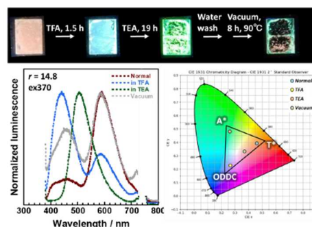
Fig. 7 Normalized fluorescence spectra of 1) ODDC-TsAPA PI film ( \lambda_{\text{ex}} = 370 nm) prepared with r = 14.8 , 2) exposed to TFA, 3) followed by exposure to TEA, and 4) finally washed with water, and the photographs of those films under UV ( \lambda = 365 nm) irradiation and its CIE coordinate.
