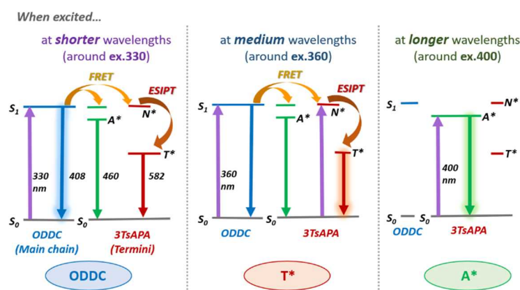
Fig. 6 Predicted photophysical processes of ODDC-TsAPA excited at shorter, medium, and longer wavelengths.
