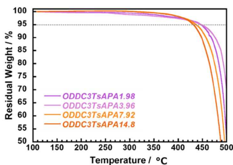
Fig. 8 Thermogravimetric analyses (TGA) for ODDC-TsAPA films prepared with variable r values ( r = 1.98, 3.96, 7.98, 14.8 ).
