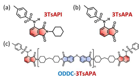
Fig. 1 Chemical structures of (a) imide compound (3TsAPI), (b) anhydride (3TsAPA), and (c) end-capped PI (ODDC-TsAPA).
