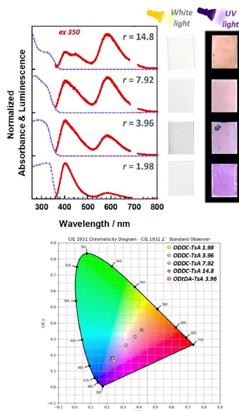
Fig. 3 UV-vis absorption and emission spectra and CIE coordinates of ODDC-TsA ( \lambda_{\text{ex}} = 350 nm), which were prepared with variable r values, and photographs of these films under white light (UV off) and UV ( \lambda = 365 nm) irradiation (UV on).
