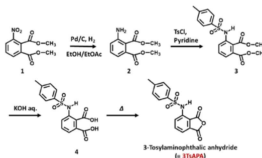
Scheme 1 Synthetic scheme of 3-tosylaminophthalic anhydride, 3TsAPA (yield : 18%).
