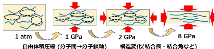
Fig. 7. Schematic image of compression of free volume and change in molecular structure by application of high pressure up to 8 GPa.
