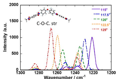
Fig. 7 FT-IR spectra (absorption bands derived from C—O—C str.) of PMDA/ODA for different \theta_{\text{C-O-C}} obtained by DFT calculation.
