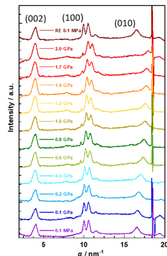
Fig. 3 Pressure-induced variations in the diffraction patterns of PMDA/ODA
