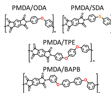
Fig. 1 Chemical structures of PIs.
