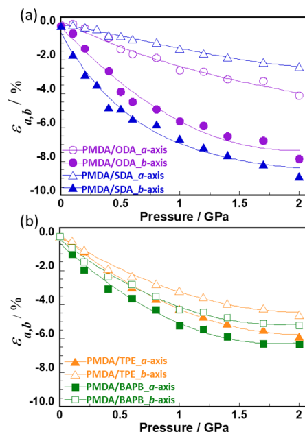
Fig. 5 Variations in \varepsilon values along the a - and b -axes of (a) PMDA/ODA and PMDA/SDA, (b) PMDA/TPE and PMDA/BAPB with increasing pressure up to 2.0 GPa.
