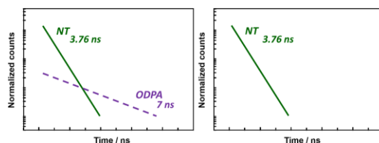
Fig. 6 Scheme of emission lifetime of NO-PI when both parts of NT and ODPa emit (left) or only part of NT emits (right).
