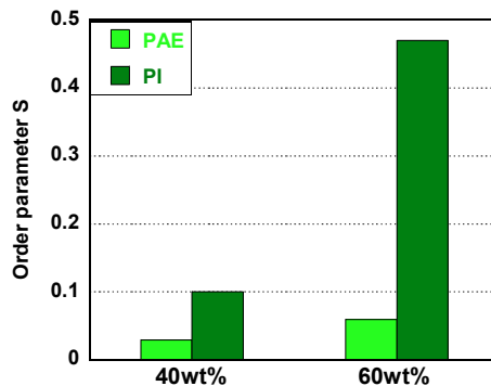
Fig. 6 Uniaxial orientation order parameter, S , for PAEs and PIs for BP4 40 wt% and 60 wt% evaluated by polarized FT-IR spectra.
