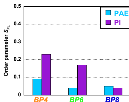
Fig.8 Uniaxial orientation order parameter, S , for PAEs and PIs evaluated from polarized fluorescence.
