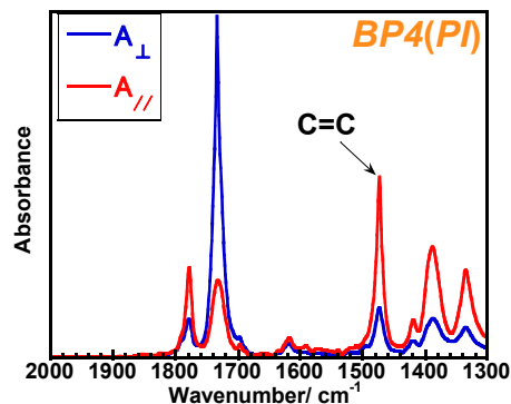
Fig. 4 Polarized FT-IR spectrum observed for shear oriented BP4 PI film with polarization direction of incident IR beam parallel (red) and perpendicular (blue) to the shear direction.
