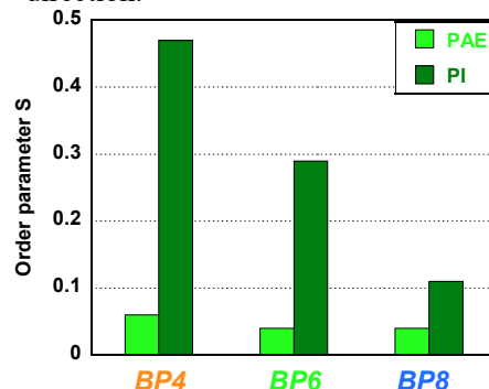
Fig. 5 Uniaxial orientation order parameter, S , for PAEs and PIs evaluated by dichroic ratio of polarized FT-IR spectra.
