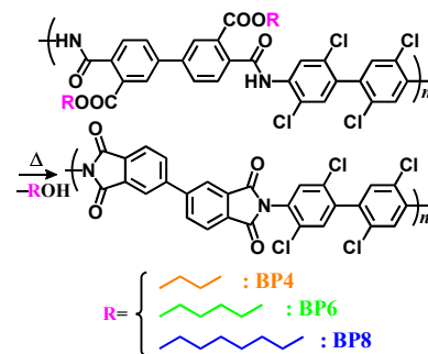
Fig. 1 Chemical structure of liquid crystalline PAE precursors and corresponding FL-PI.
