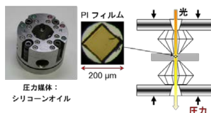
Fig. 3 Diamond anvil cell, photo of a sample, and schematic view of
