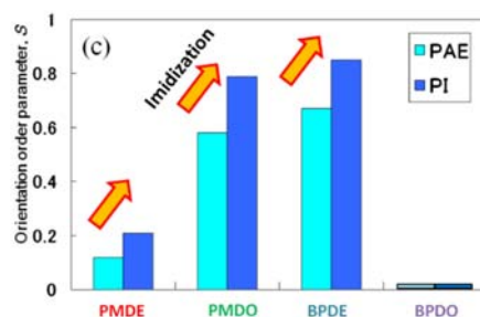
Fig. 4 WAXD patterns of (a) BPDE (PAE), (b) BPDE (PI). (c) Orientation order parameter, S of PAEs and resultant PIs
