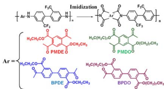
Fig. 1 Chemical structures of PAEs and resultant PIs
