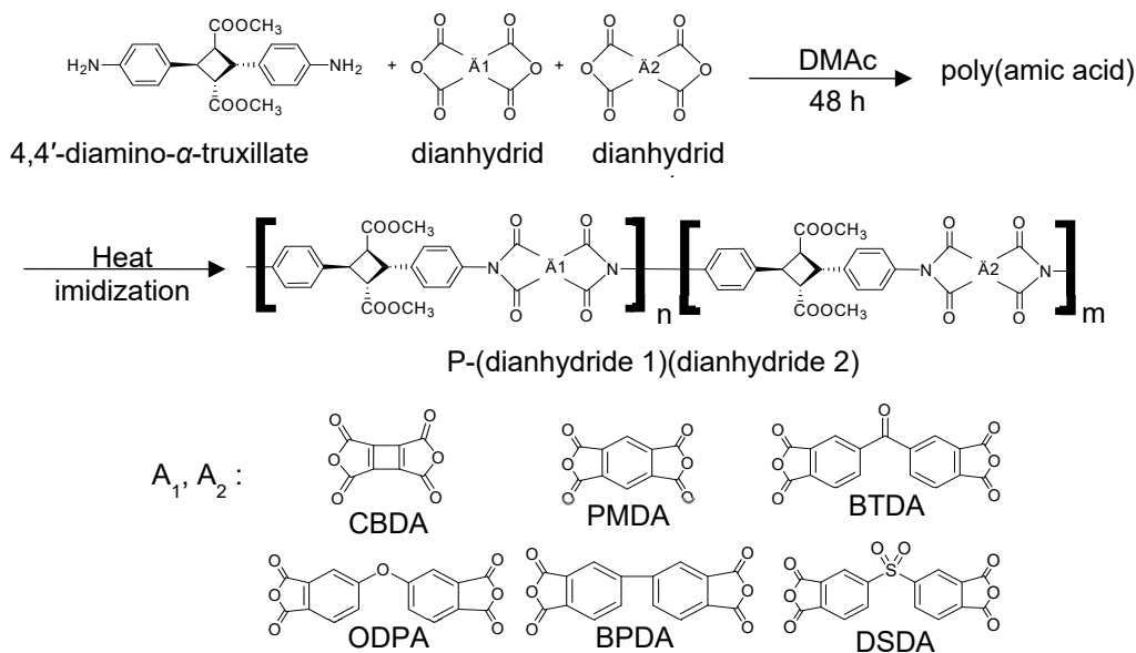
Scheme 1. Synthetic route and chemical structures of BPI polymers derived from 4,4'-diamino- \alpha -truxillate with dianhydrides
