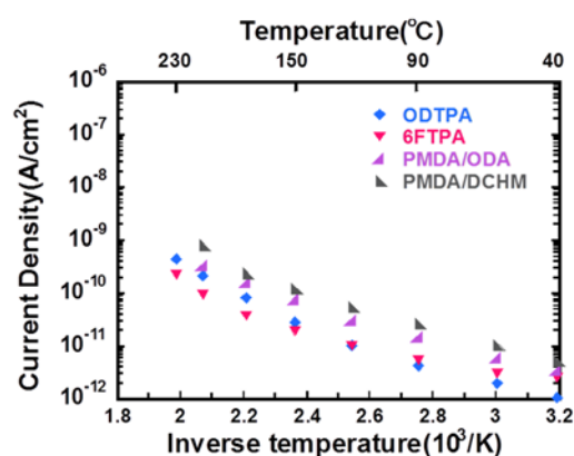
Fig. 4 Temperature dependence of current density in ODTPA, 6FTPA
