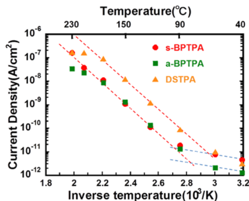
Fig. 3 Temperature dependence of current density in s -BPTPA, a -BPTPA, DSTPA
