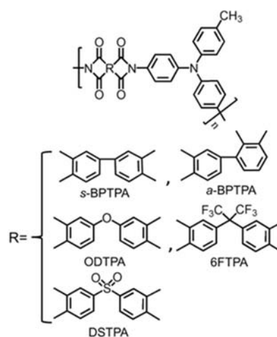
Fig. 1 Chemical structures of PIs.
