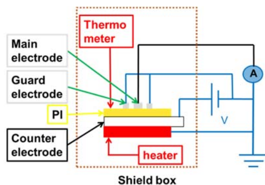
Fig. 2 Experimental setup for dark-current measurements.
