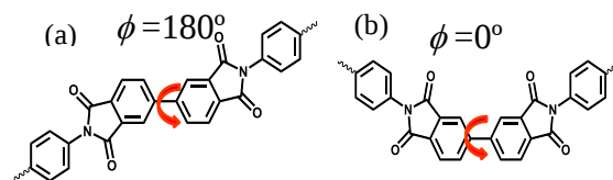
Fig. 3 Conformations at (a) \phi=180^\circ and (b) \phi=0^\circ .
